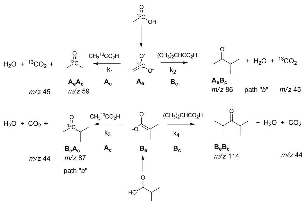
Scheme 2. Product Distribution and Pathways for the Cross-Ketonization Reaction of Isobutyric Acid, B, with Acetic Acid, A, Having 13 C Labeled Carbonyl Group a
