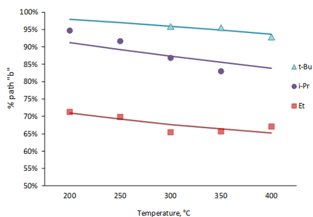
Figure 3. Preference for Path "b" depending on temperature for different acids with KOH treated ZrO_2 catalyst. Dots represent measured data. Solid lines represent the linear trendlines serving as the basis for the calculation of the activation energy difference between two pathways.
